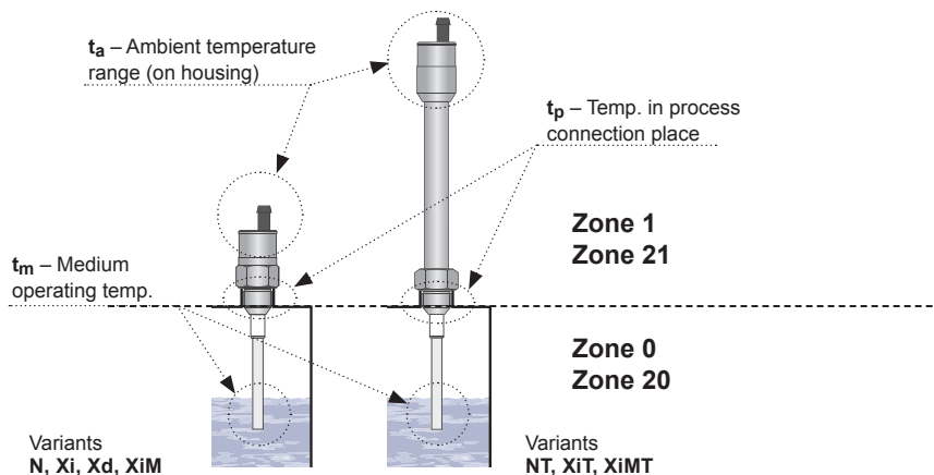
Fig. 15: Places for measurement of temperature and explosive areas
