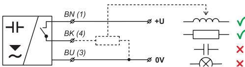
Fig. 14: PNP type sensors connection (version "N", "NT", "Xd")
