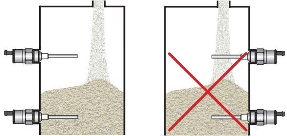
Fig. 3: Side wall mounting
