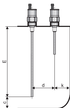
Fig. 1: Vertical mounting
