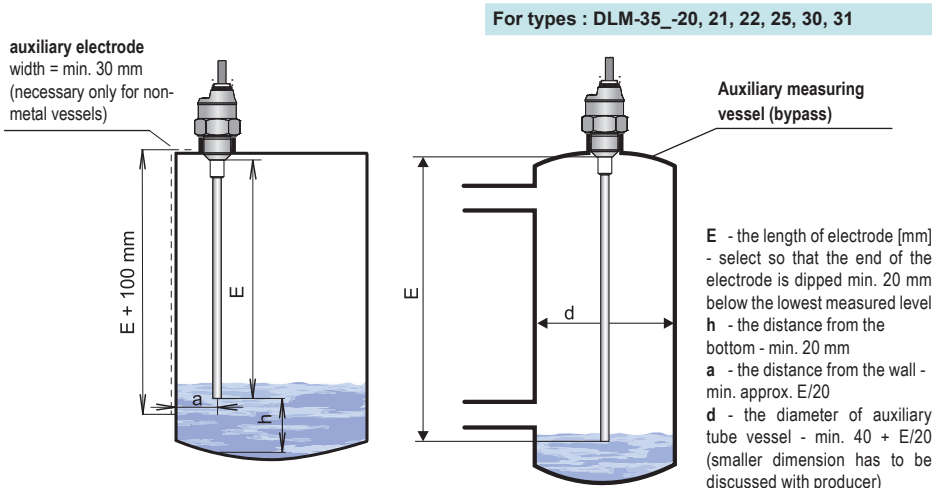
Fig. 1: Installation of level meters with rod electrode
