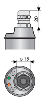
Variant "D" with dustproof cable outlet
