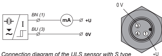
Fig. 22: Connection diagram of the ULS sensor with S type output (two-state current switch 44\text{ mA} / 20\text{ mA} )
