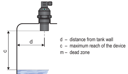
Fig. 3: Distance of the device from the tank wall
