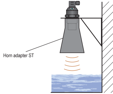
Fig. 14: Horn adapter installation
