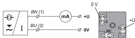
Fig. 15: Connection diagram of the ULM level meter (variant -I) and inside view of the connector
