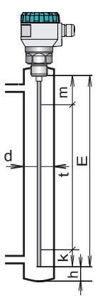
Fig. 5: Level meter installation into the auxiliary vessel
