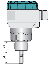
Fig. 19: Level meter without electrode
