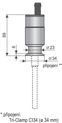
Tri-clamp
