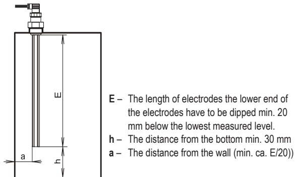
Fig. 5: Installation of level meter with reference electrode
