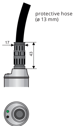
Variant "H" with gland for protected hoses - for use in outdoor environments or in areas with increased moisture.
