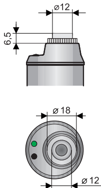
Variant "A" with short stainless steel gland
