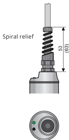
Variant "V" with plastic gland with spiral relief - in case of increased mechanical strain on the cable.
