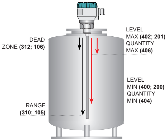
Fig. 1: Basic level meter commands
