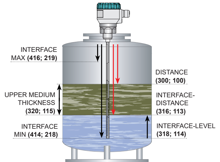
Fig. 2: Level and interface measurement
