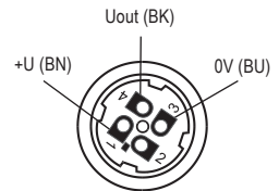
Fig. 6: Inside of the connector socket (variant "C")
