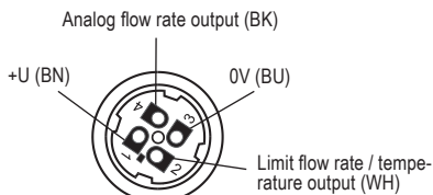
Fig. 9: Inside view of the connector socket (variant "C-IFPF(P)")
