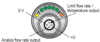
Fig. 7: Connector of flow sensor TFS-35_...-IFPF and TFS-35_...-IFPT
