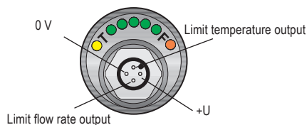
Fig. 6: Connector of flow sensor TFS-35_...-PFPT
