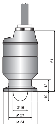
RFLS-35_-2-C134 (Tri-clamp)
