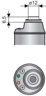
Variant "V" with plastic cable gland with spiral relief – in case of increased mechanical wear on the cable.
