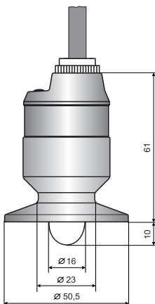
RFLS-35_-2-C150 (Tri-clamp)
