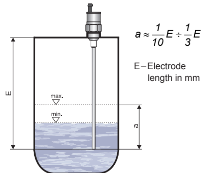
Fig. 11: Two state regulation by hysteresis setting
