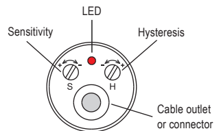
Fig. 17: Top view of level sensor
