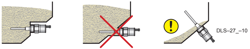
Fig. 5: Slant wall mounting
