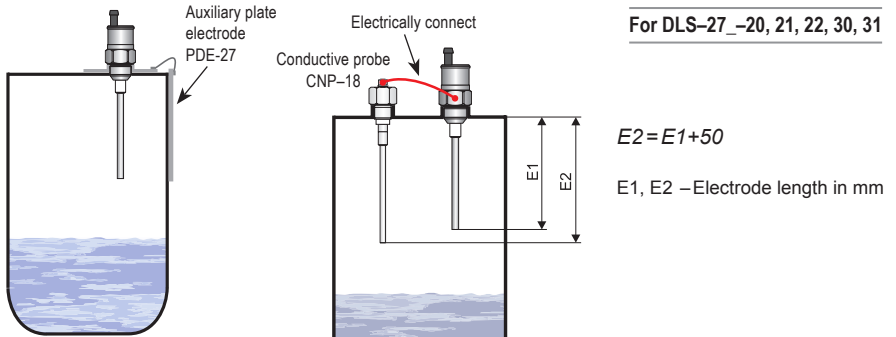
Fig. 6: Auxiliary electrode in non-conductive tanks
