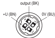
Fig. 16: Inside of the connector socket
