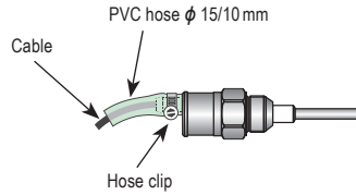
Fig. 9: Protective hose install
