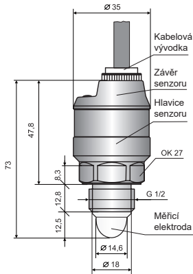
RFLS-35_-2-G1/2
