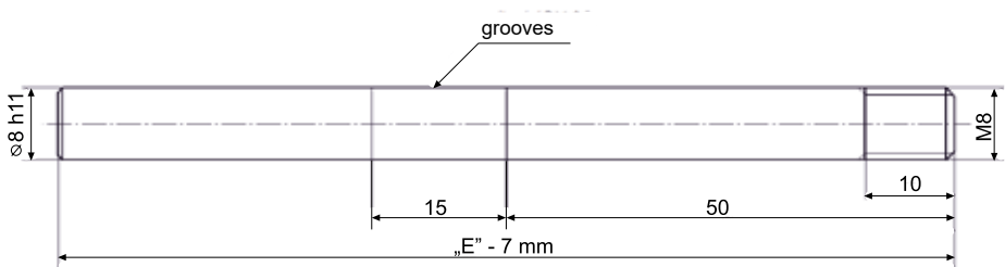
Fig. 23: Detail of a drawing of a rod electrode
