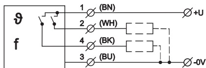
Fig. 4: Connection of flow sensor TFS-35_...-PFPT
