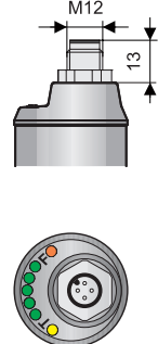
Variant „C“ with connector M12
