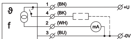
Fig. 5: Connection of flow sensor TFS-35_...-IFPF and TFS-35_...-IFPT
