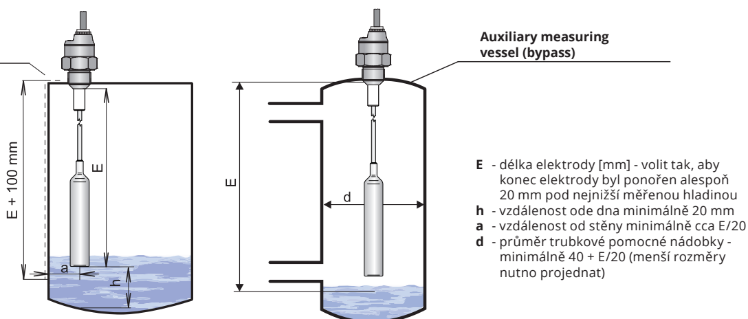
Fig. 20: Installation of level meters with insulated rope electrode
