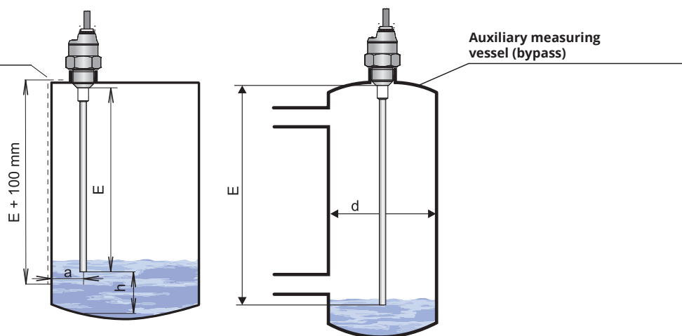
Fig. 19: Installation of level meters with rod electrode
