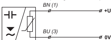
Fig. 13: Connection of a sensor with a NAMUR type output (configuration Xi, XiM, XiT, XiMT)
