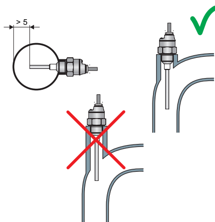
Fig. 8: Sensor mounting in a tube
