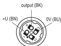
Fig. 14: Inside of the connector socket
