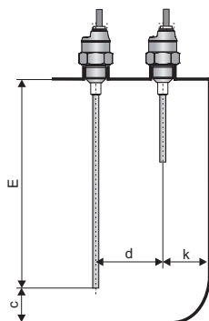
Fig. 1: Vertical mounting
