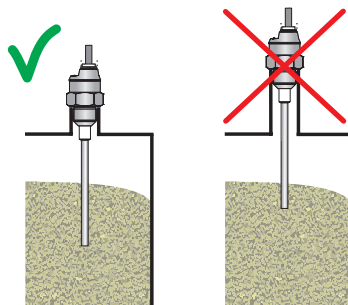
Fig. 10: Long fitting tubes in vertical mounting
