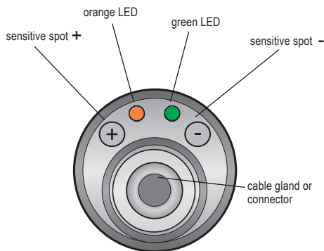
Fig. 15: Top view of sensor control elements
