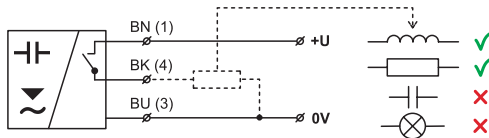
Fig. 9: PNP type sensors connection (version "P")
