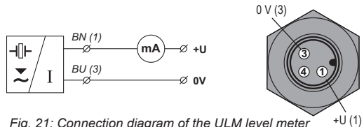
Fig. 21: Connection diagram of the ULM level meter (variant -I) and view of the connector
