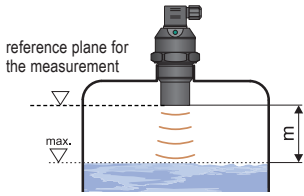
Fig. 2: Dead zone of the device
