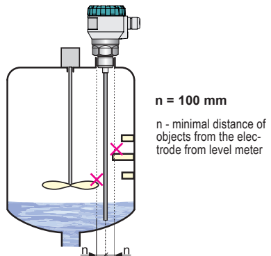
Fig. 13: Incorrect level meter installation close to obstacles
