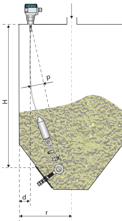
Obr. 19: Recommended Level meter installation with anchorage
