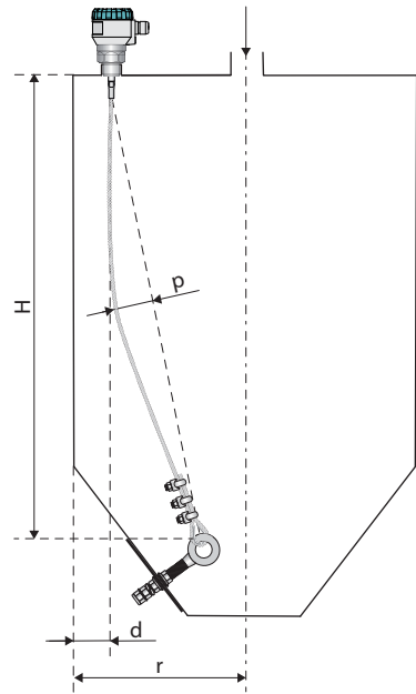
Fig. 21: Recommended installation of the level meter with anchoring on the same side of the silo
