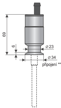
Tri-clamp
