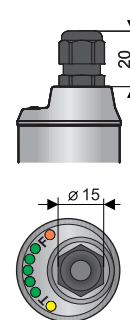
Variant "C" with connector M12
