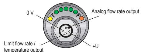
Connector of flow sensor TFS-35_ _ _ -IFPF and TFS-35_ _ _ -IFPT
