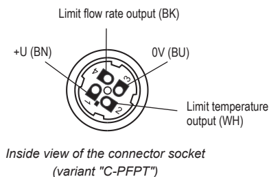
Connector of flow sensor TFS-35_ _ _ -PFPT
