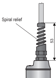
Variant "V" with plastic cable gland with spiral relief - for case of increased mechanical wear on the cable.
