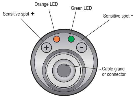
Fig. 7: Top view of level sensor
