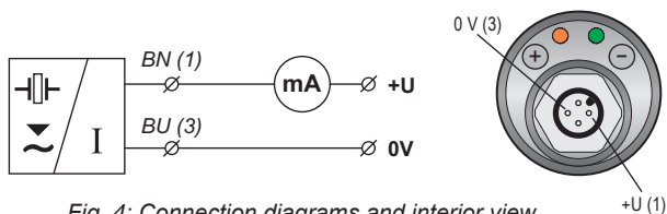
Fig. 4: Connection diagrams and interior view of connector of level meter DLM (variant - I)
