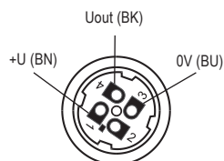
Fig. 6: Inside of the connector socket (variant "C")
