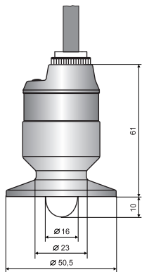
RFLS-35_-2_-CI50 (Tri-clamp DIN 32676)
