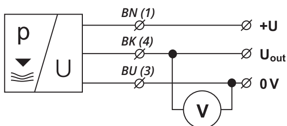
Connection diagram and internal view of the PPM-35 sensor connector (U variant)
