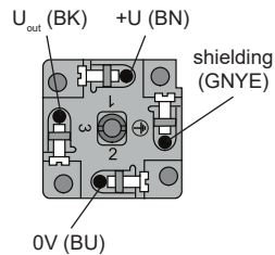
Fig. 9: Internal view of the connector with voltage output
