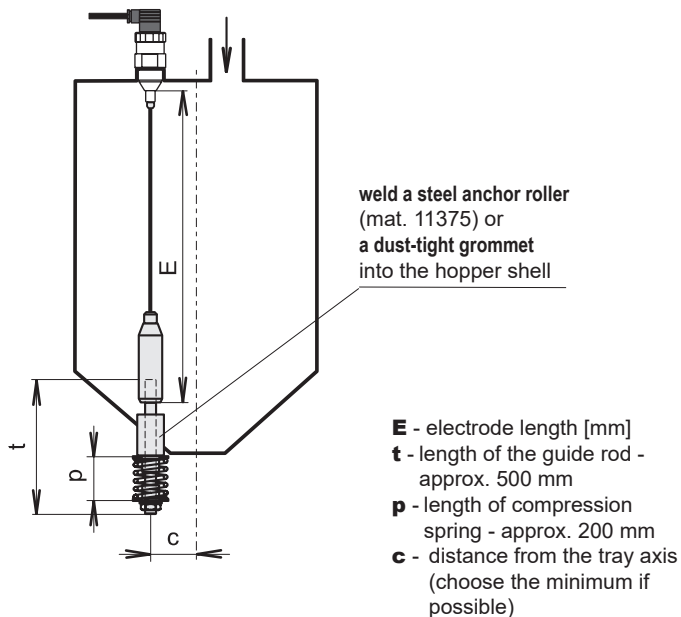
Fig. 4: Installation of the level meter with rope electrode and anchoring
