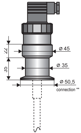
Tri-Clamp process connection
