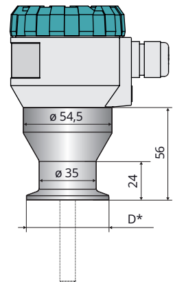
Tri- Clamp
