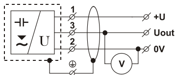
Fig. 8: Connection diagram of the level meter with voltage output
