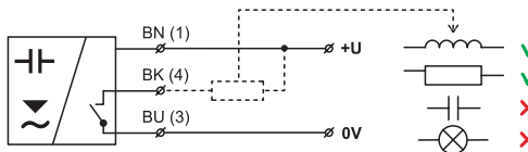
Fig. 7: NPN type sensors connection (version "N")
