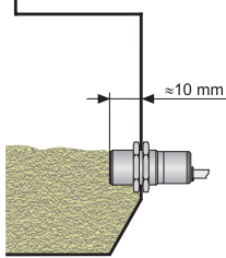
Fig. 1: Sensing bulky-solid materials in storage tanks
