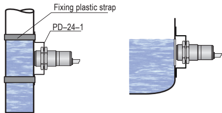
Fig. 4: CPS sensor application for level gauges and eye sights
