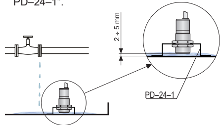
Fig. 2: Use of CPS for sensing leakages in an interception tank
