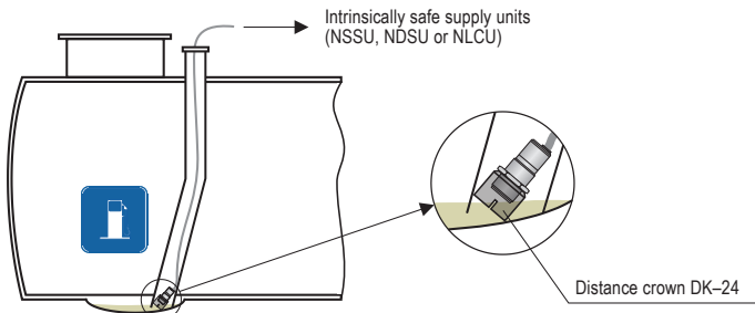
Fig. 5: Use of CPS for indicating presence of liquid in the inter-wall space
