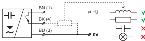
Fig. 9: PNP type sensors connection (version "P")
