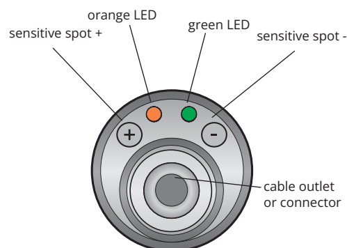
Fig. 26: Top view of level meter
