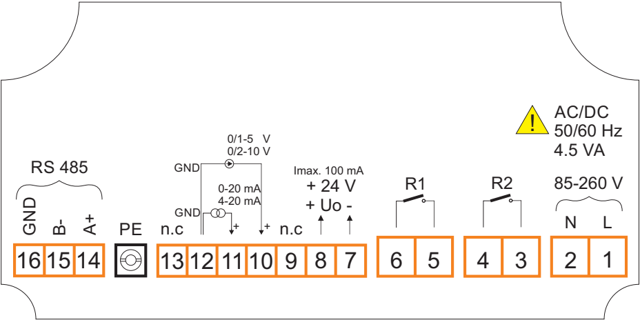
Fig. 2: Terminal description
