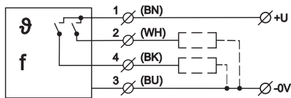
Connection of flow sensor TFS-35_--_--PFPT
