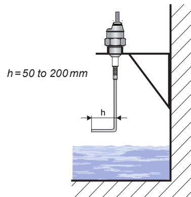
Bending of the electrode end to sense unknown fluids
