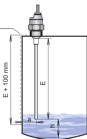
Fig. 19: Installation of level meters with rod electrode
